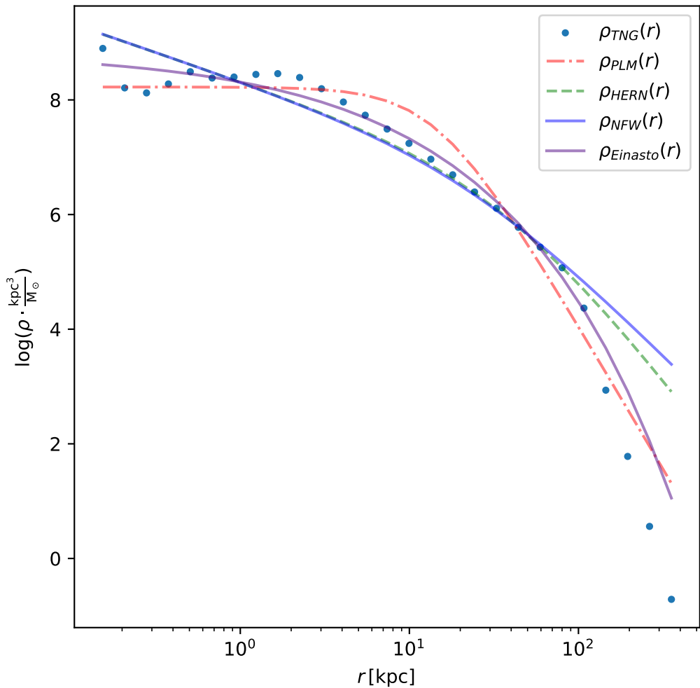
Radial Density Profile of Dark Matter Subhalo
