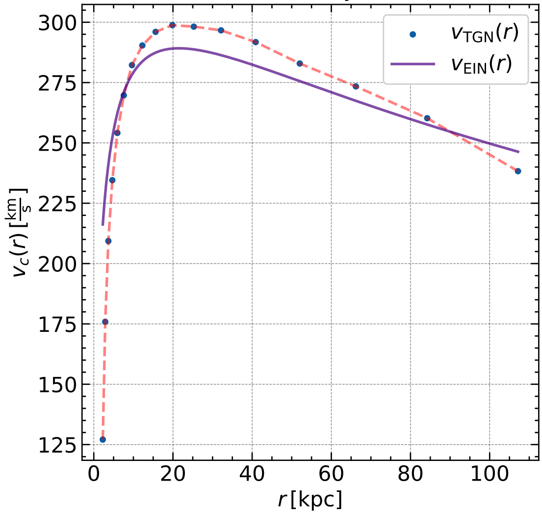
Circular Velocity Profile
