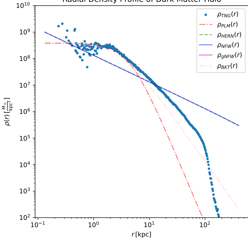
Radial Density Profile of Dark Matter Halo
