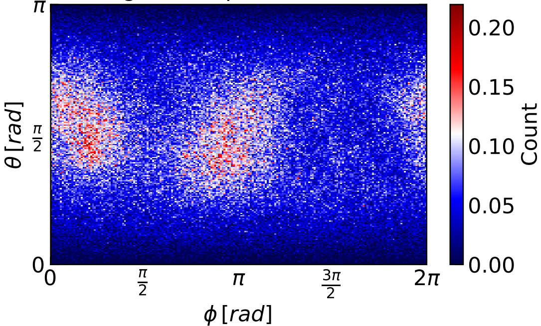
2D Histogram in Spherical Coordinates
