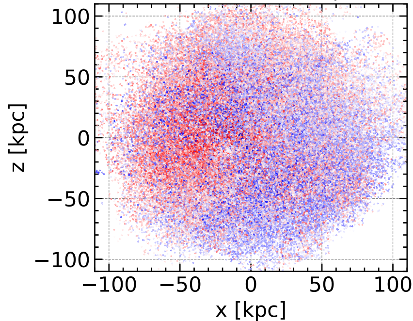
DM distribution in xz-plane
