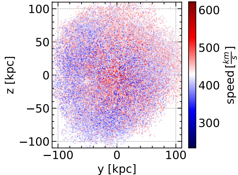
DM distribution in yz-plane
