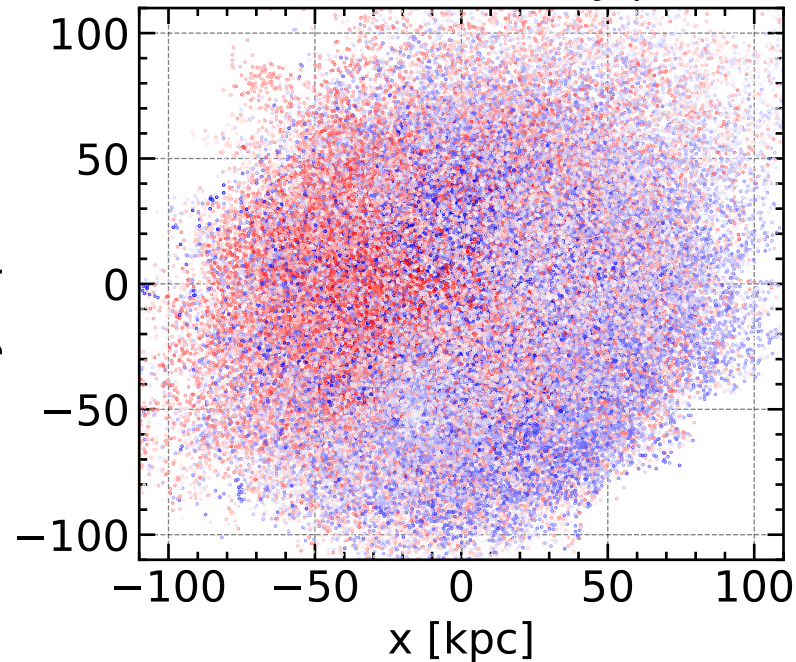
DM distribution in xy-plane
