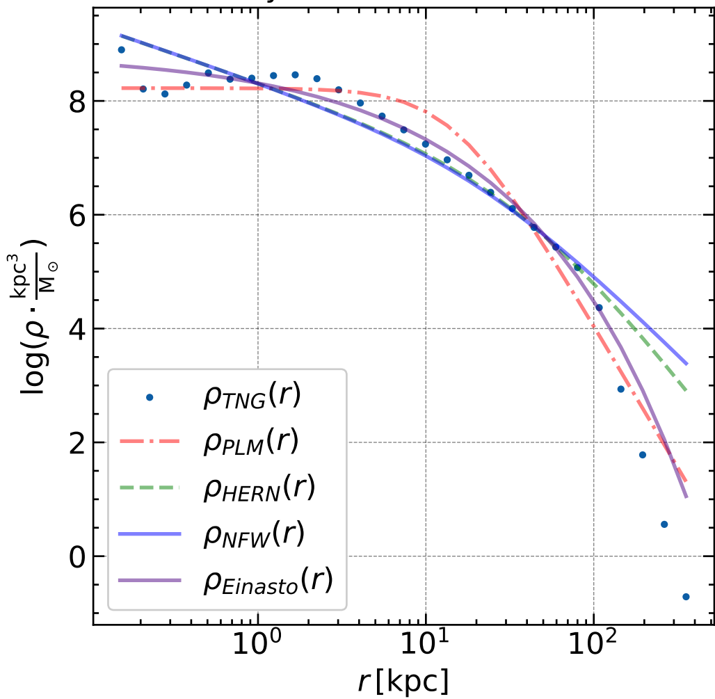
Radial Density Profile of Dark Matter Subhalo
