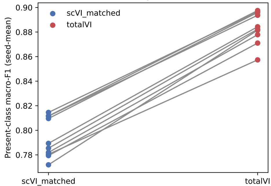
Lawlor donor-paired macro-F1
