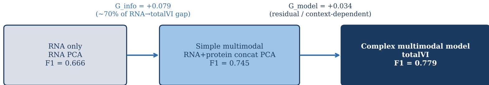
Figure 1. Central logic: information gain vs model-specific advantage
