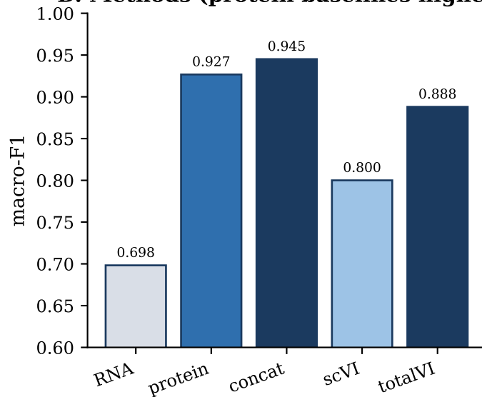
D. Methods (protein baselines highest)
