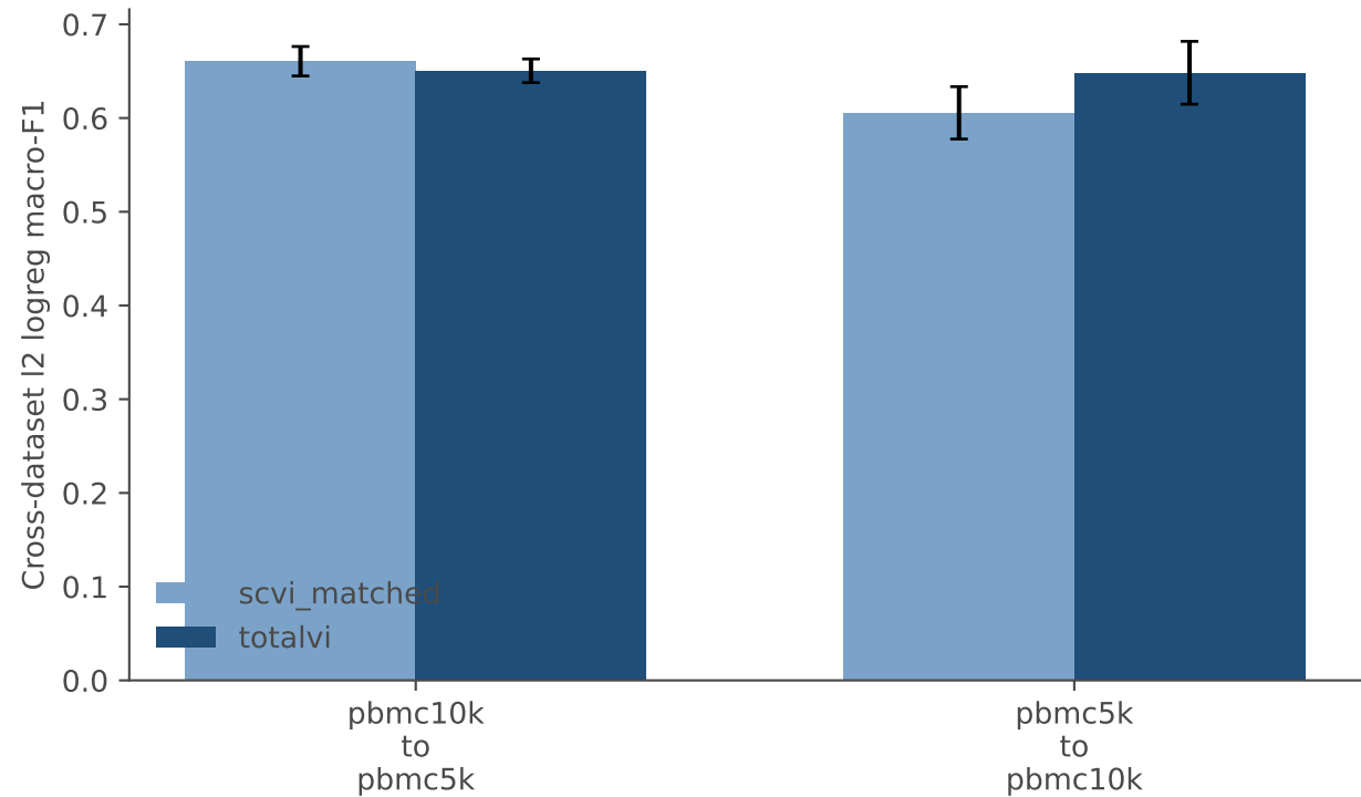
High-confidence I2 transfer performance
