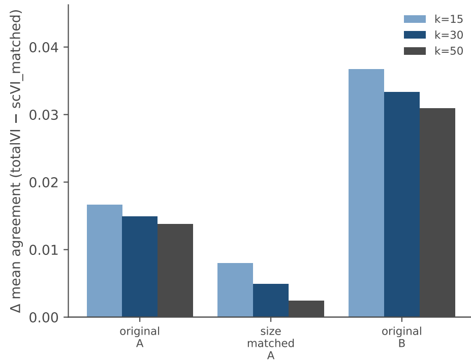
l2 neighbor label agreement
