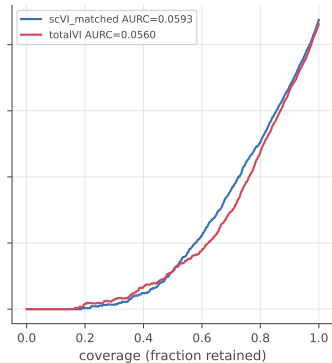
B: PBMC5k \rightarrow PBMC10k
