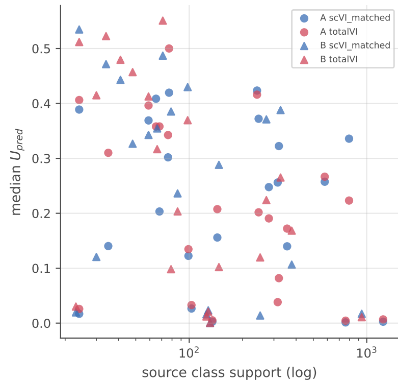
Source class support vs uncertainty and error (per l2 class)
