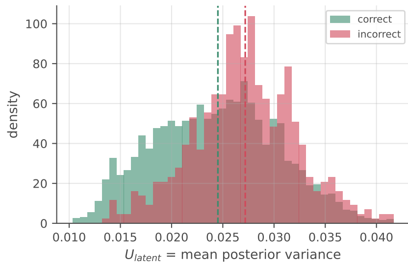
Figure 4. Target latent posterior uncertainty: correct vs incorrect (seed 0)
