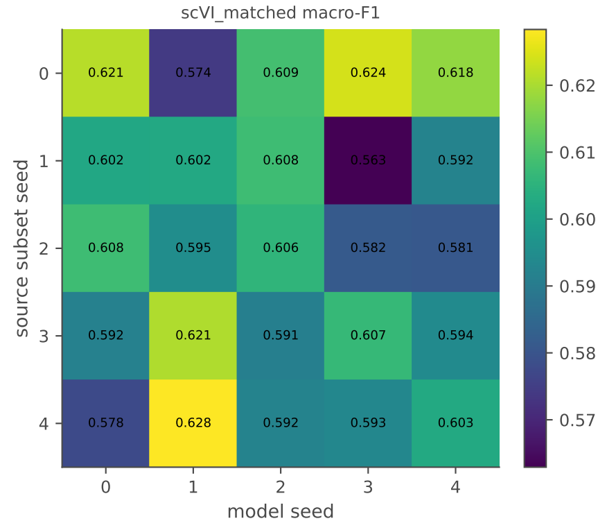
Figure 7. Crossed source-subset x model-seed I2 macro-F1 (Direction A)
