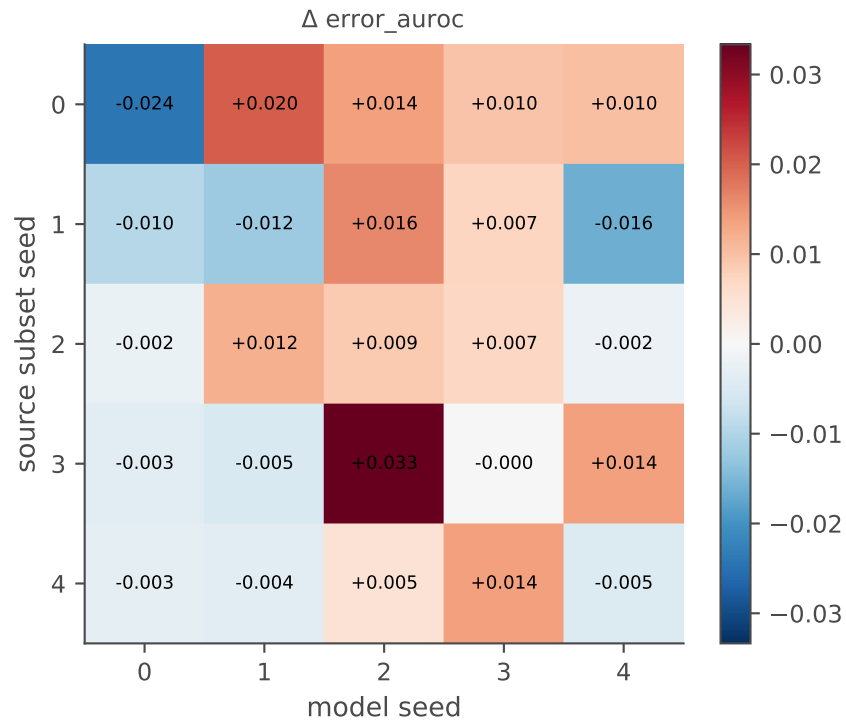
Figure 8. \Delta = \text{totalVI} - \text{scVI\_matched} across the crossed grid
