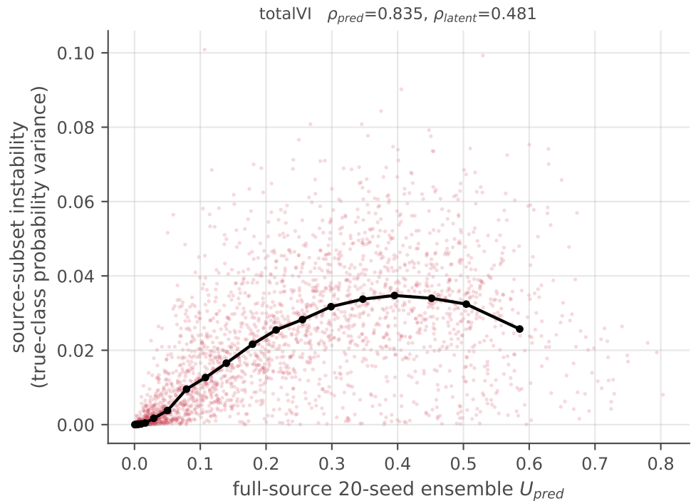
Figure 11. Full-model uncertainty versus source-subset instability (black: 20-quantile medians)
