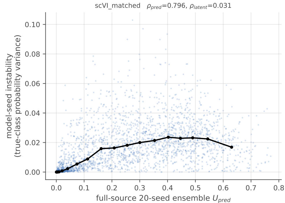
Figure 12. Full-model uncertainty versus model-seed instability (black: 20-quantile medians)
