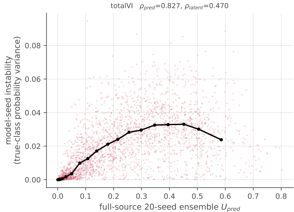
Figure 12. Full-model uncertainty versus model-seed instability (black: 20-quantile medians)
