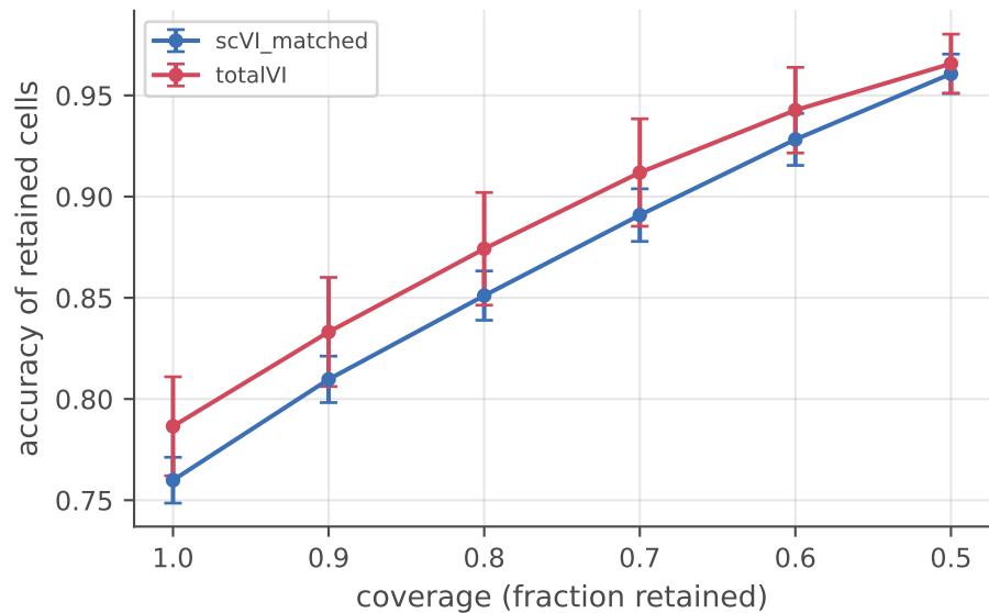
Figure 13. Selective prediction across 20 seeds (mean \pm SD)
