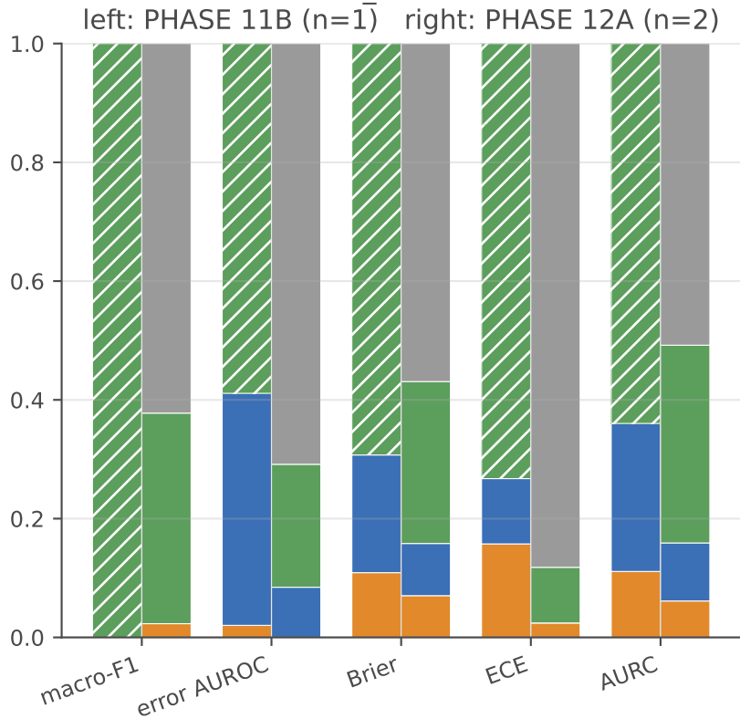
Figure 1b. Replication splits the PHASE 11B interaction/residual term
