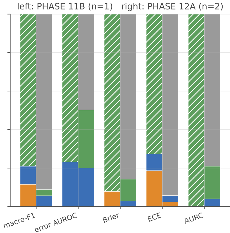
Figure 1b. Replication splits the PHASE 11B interaction/residual term
