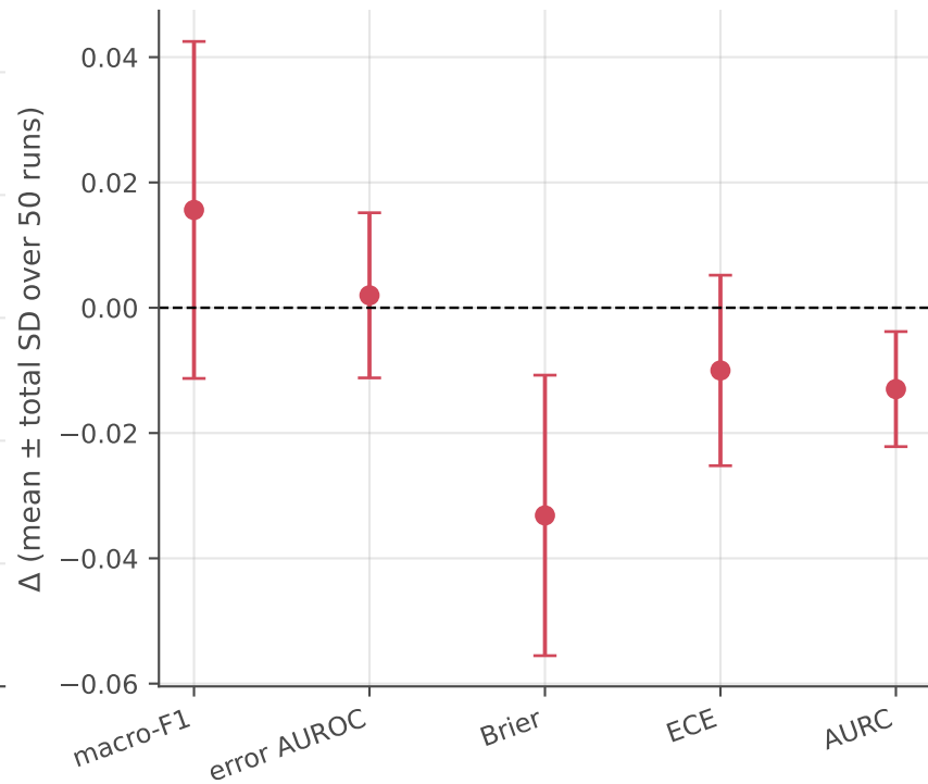
Figure 3. Decomposition of the totalVI – scVI difference
