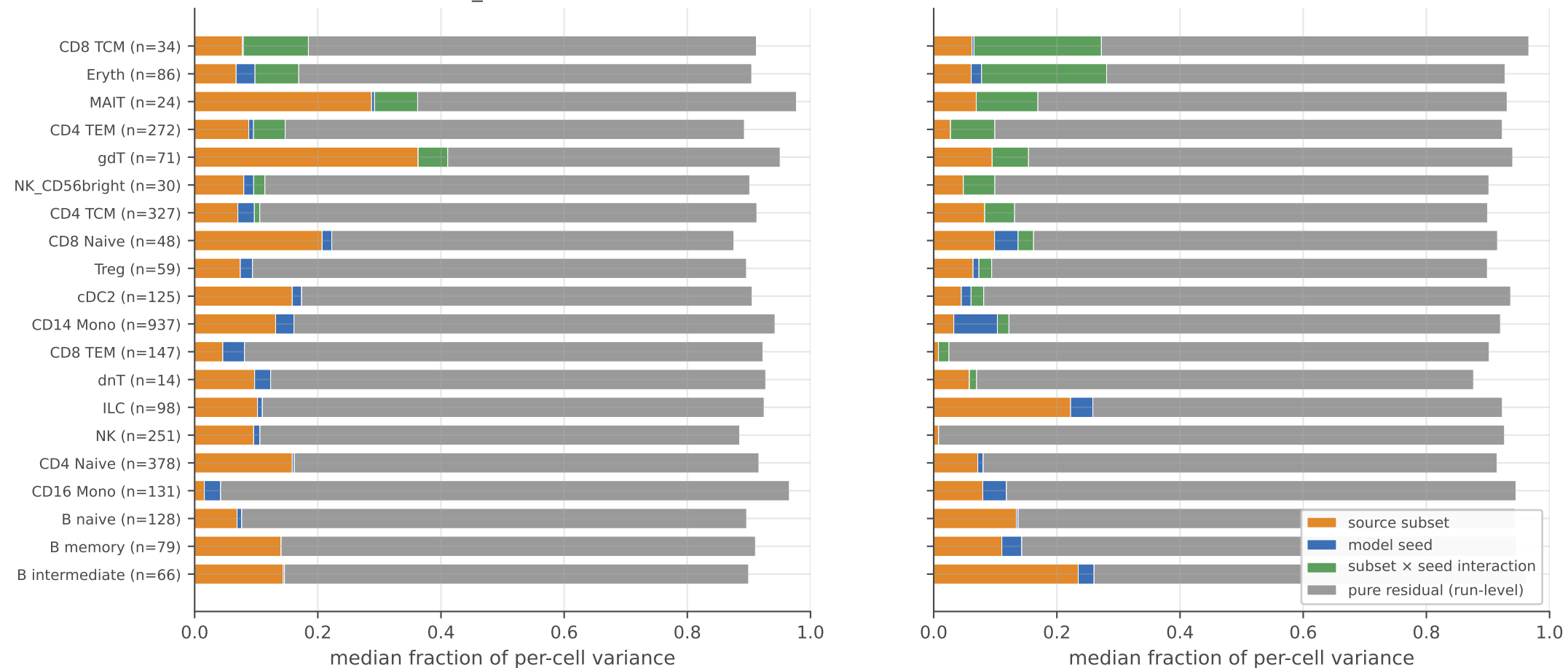
Figure 4. Per-cell-type variance decomposition (true-class probability, 5 \times 5 \times 2 design)
