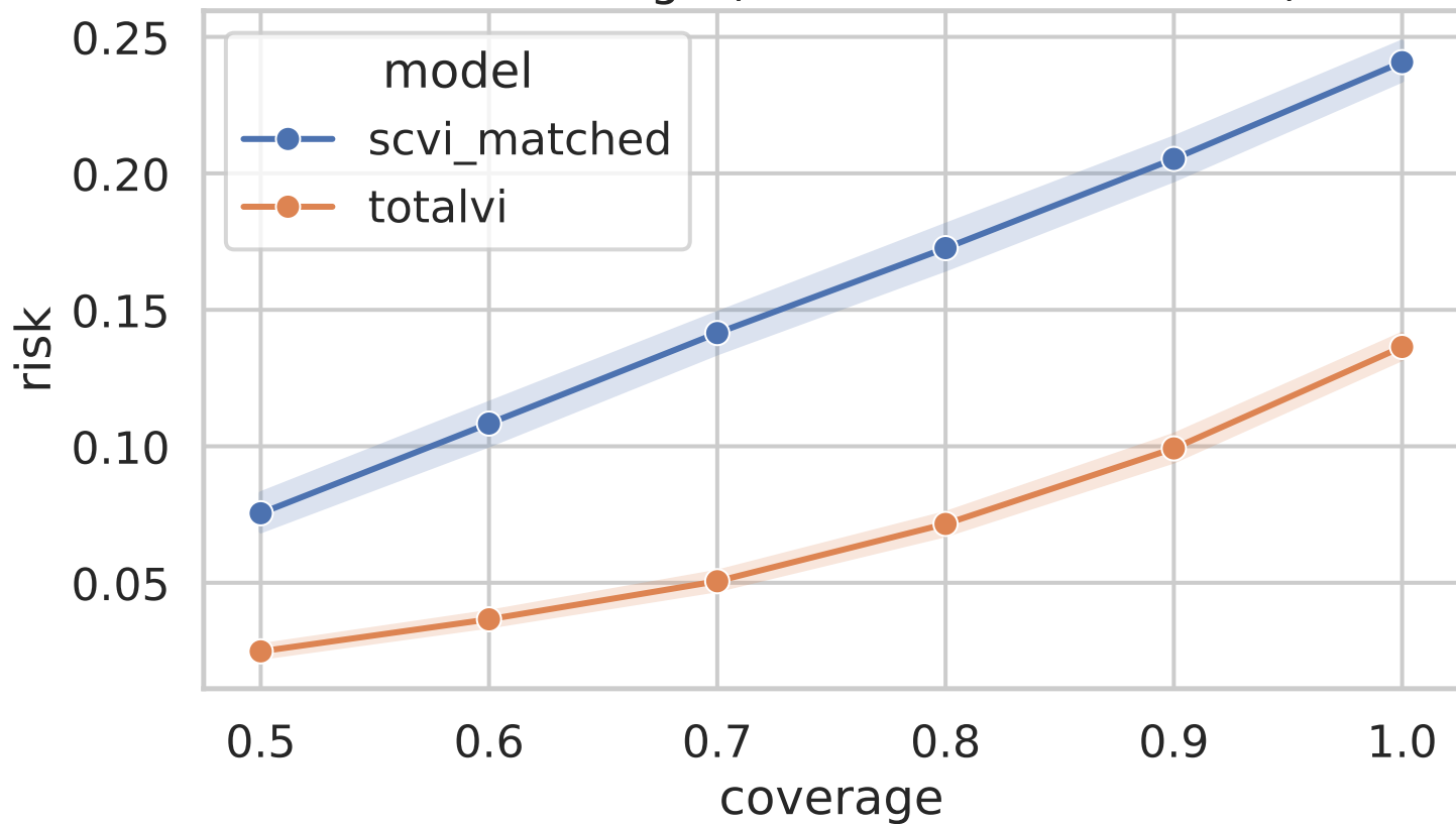
Risk-coverage (confidence abstention)
