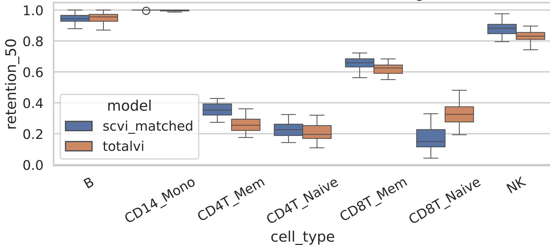
Per-class retention at 50% coverage
