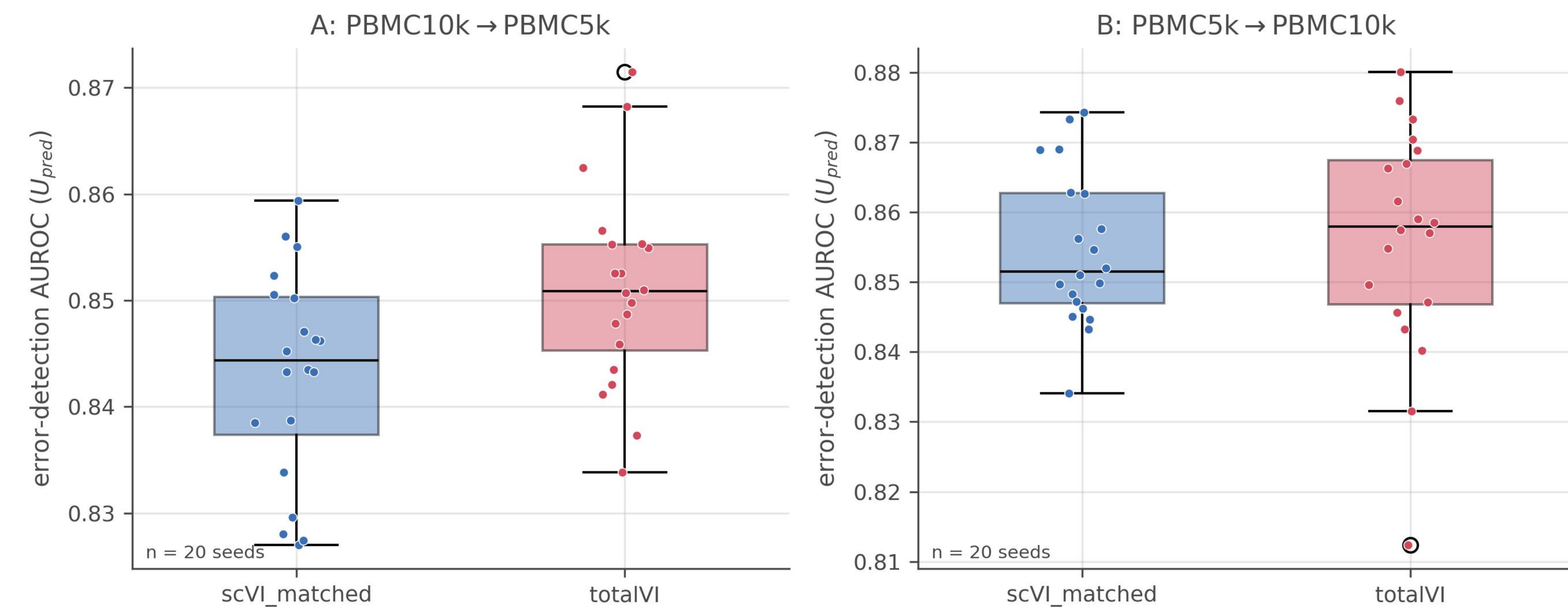
Figure 2. 20-seed distribution of predictive error-detection AUROC
