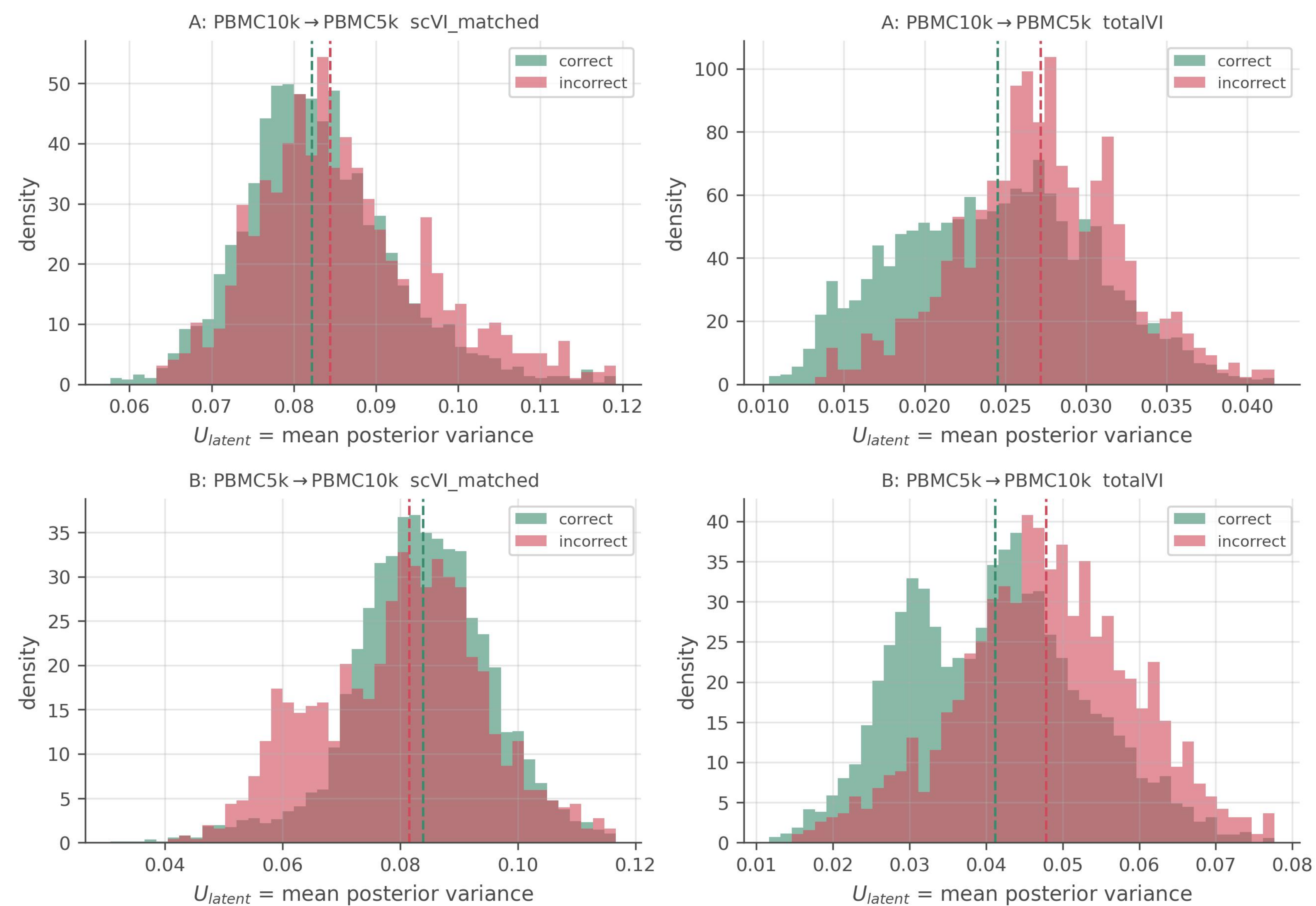
Figure 4. Target latent posterior uncertainty: correct vs incorrect (seed 0)
