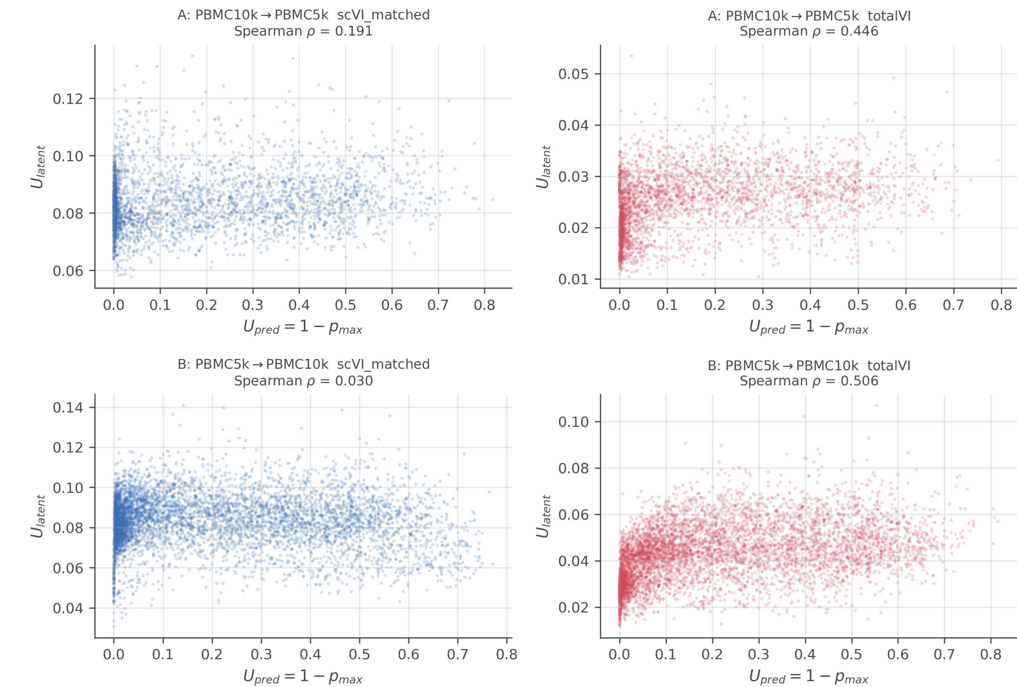
Figure 5. Predictive versus latent posterior uncertainty (seed 0)
