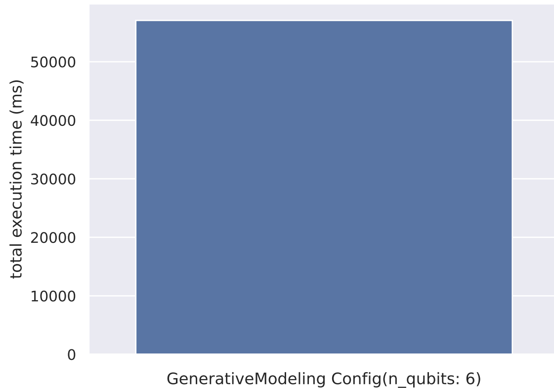
GenerativeModeling
