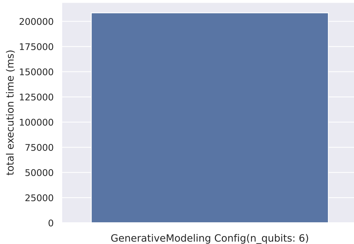
GenerativeModeling
