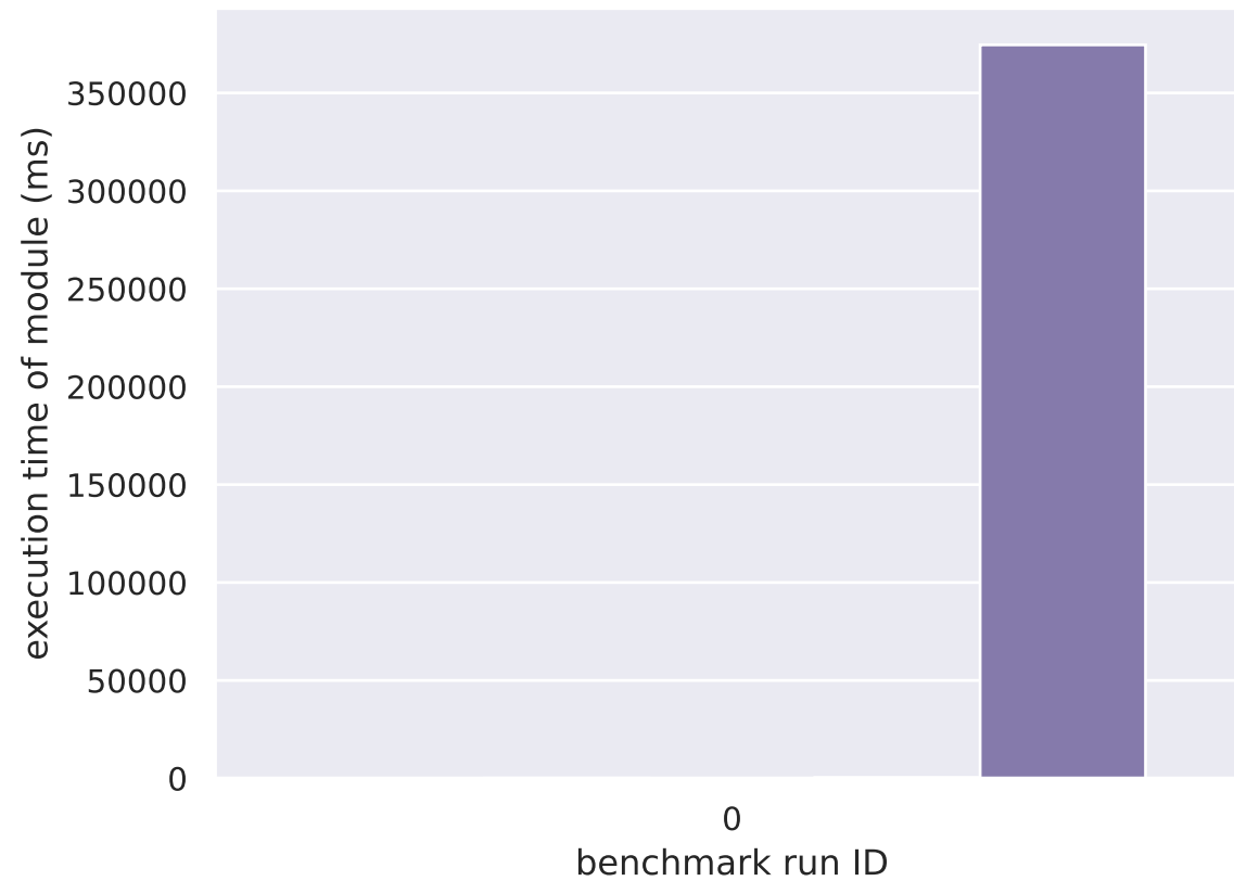
GenerativeModeling
