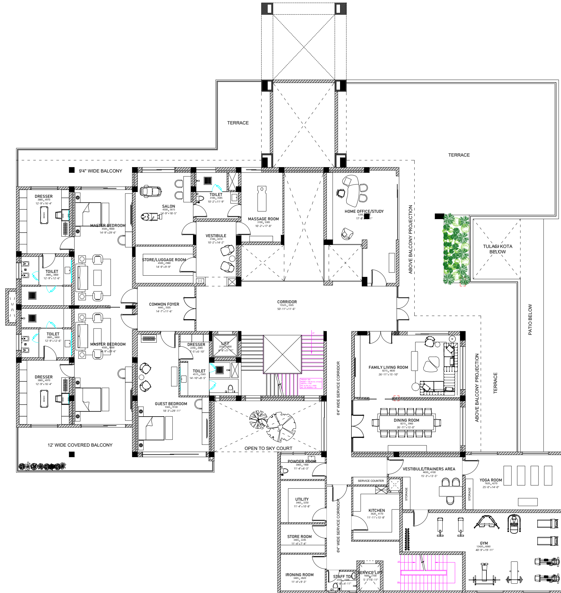
E-6,VILLA-01,FIRST FLOOR PLAN
