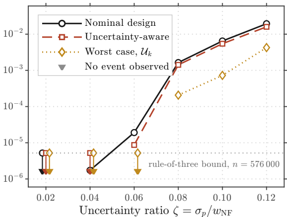
Outage probability
