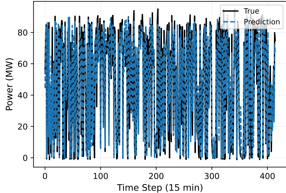
FLSVR vs True (Wind farm site 6 (Nominal capacity-96MW)) Segment [0, 415)
