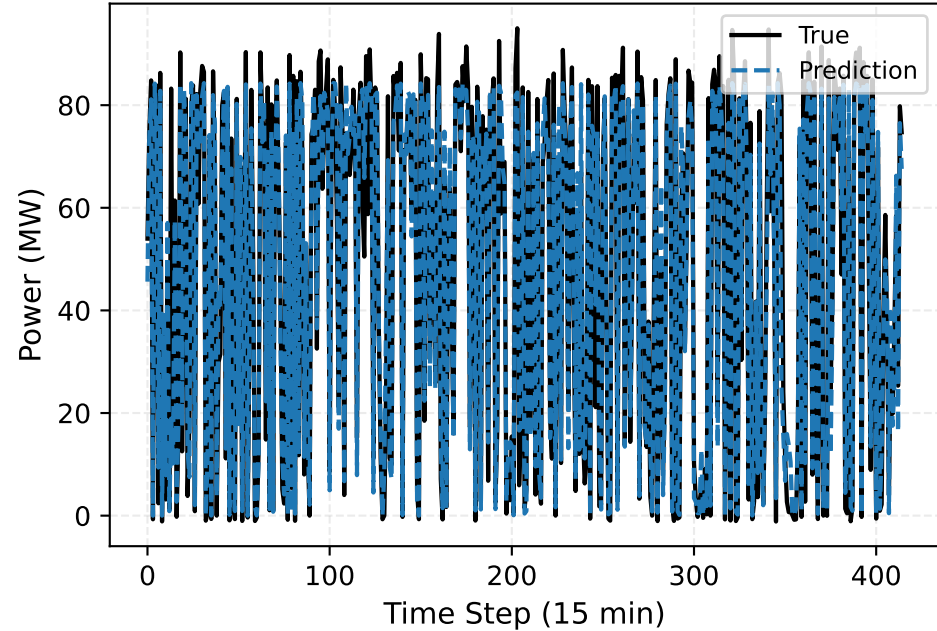
RF-WPF vs True (Wind farm site 6 (Nominal capacity-96MW)) Segment [0, 415)
