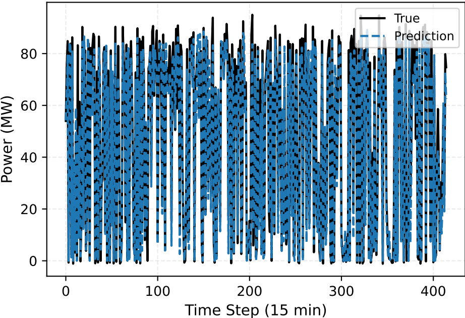
TL-QLDMR vs True (Wind farm site 6 (Nominal capacity-96MW)) Segment [0, 415)
