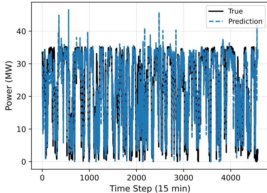
ELM vs True (Wind farm site 5 (Nominal capacity-36MW))
