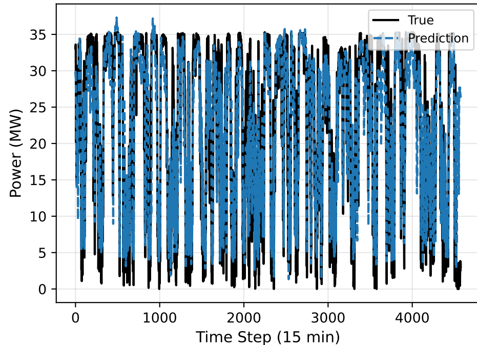
TL-LSTM vs True (Wind farm site 5 (Nominal capacity-36MW))
