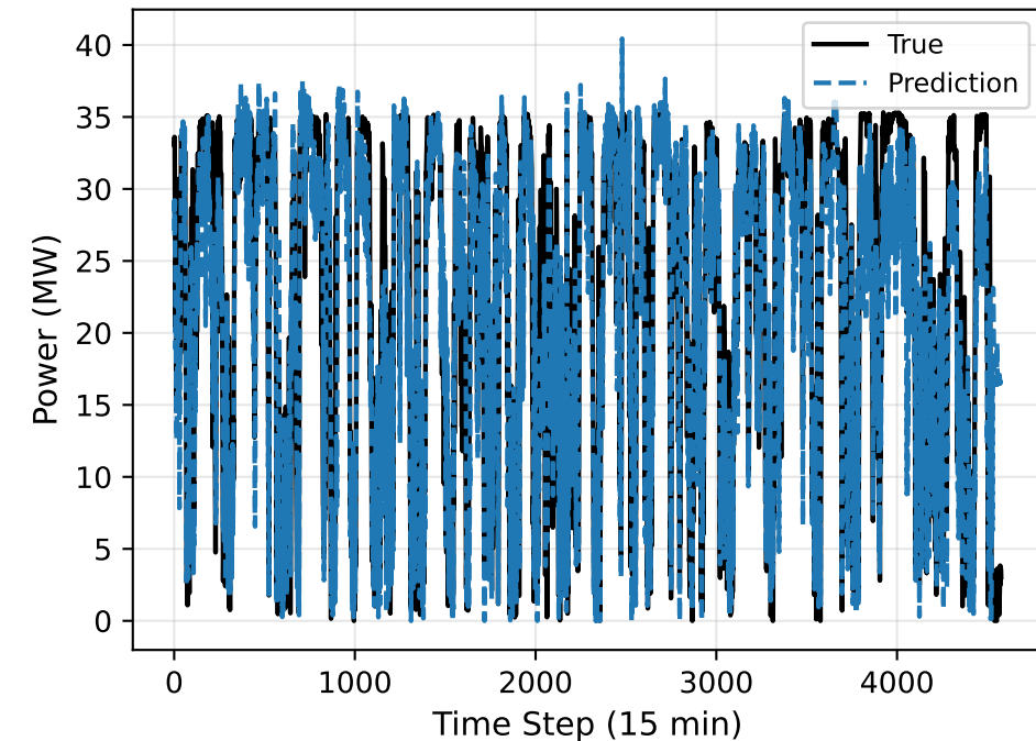
QLDMR(Median) vs True (Wind farm site 5 (Nominal capacity-36MW))
