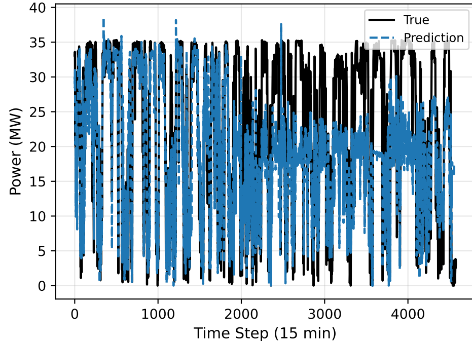
TL-SVR vs True (Wind farm site 5 (Nominal capacity-36MW))
