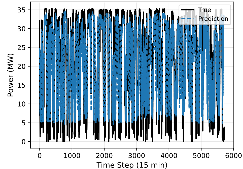
CNN-LSTM vs True (Wind farm site 5 (Nominal capacity-36MW))
