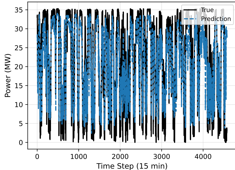
CNN-LSTM vs True (Wind farm site 5 (Nominal capacity-36MW))
