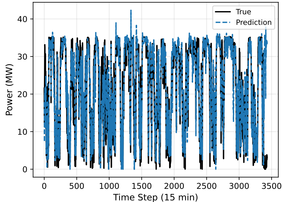
SVR vs True (Wind farm site 5 (Nominal capacity-36MW))
