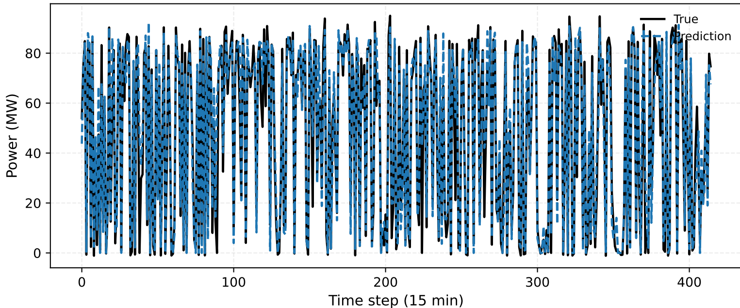
ARA-SVR vs True (Wind farm site 6 (Nominal capacity-96MW)) | Local segment [0, 415)
