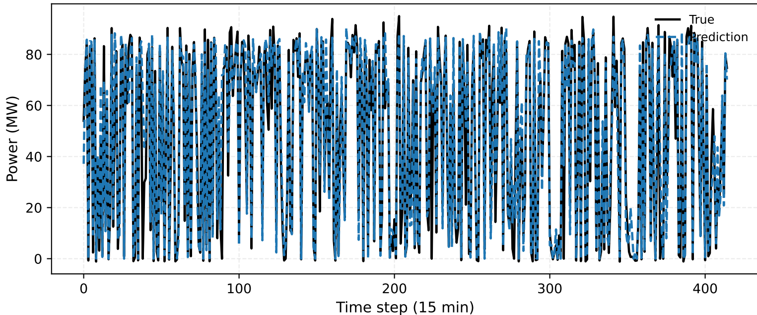
BLSSVR vs True (Wind farm site 6 (Nominal capacity-96MW)) | Local segment [0, 415)
