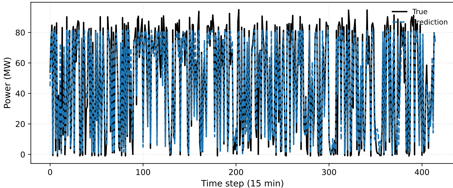
BRF-WPF vs True (Wind farm site 6 (Nominal capacity-96MW)) | Local segment [0, 415)
