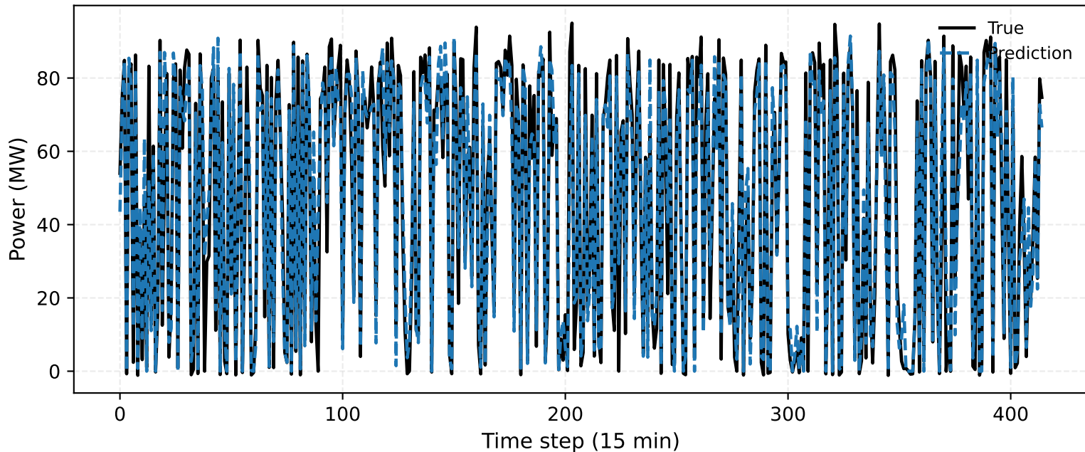
FLSVR vs True (Wind farm site 6 (Nominal capacity-96MW)) | Local segment [0, 415)
