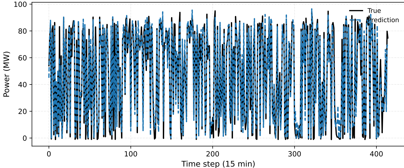
HHO-SVR vs True (Wind farm site 6 (Nominal capacity-96MW)) | Local segment [0, 415)
