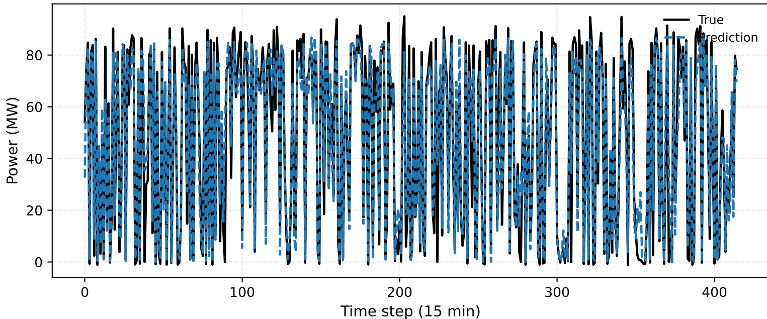
KMeans-GBT vs True (Wind farm site 6 (Nominal capacity-96MW)) | Local segment [0, 415)
