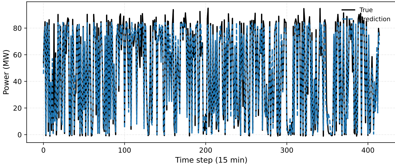
RF-WPF vs True (Wind farm site 6 (Nominal capacity-96MW)) | Local segment [0, 415)
