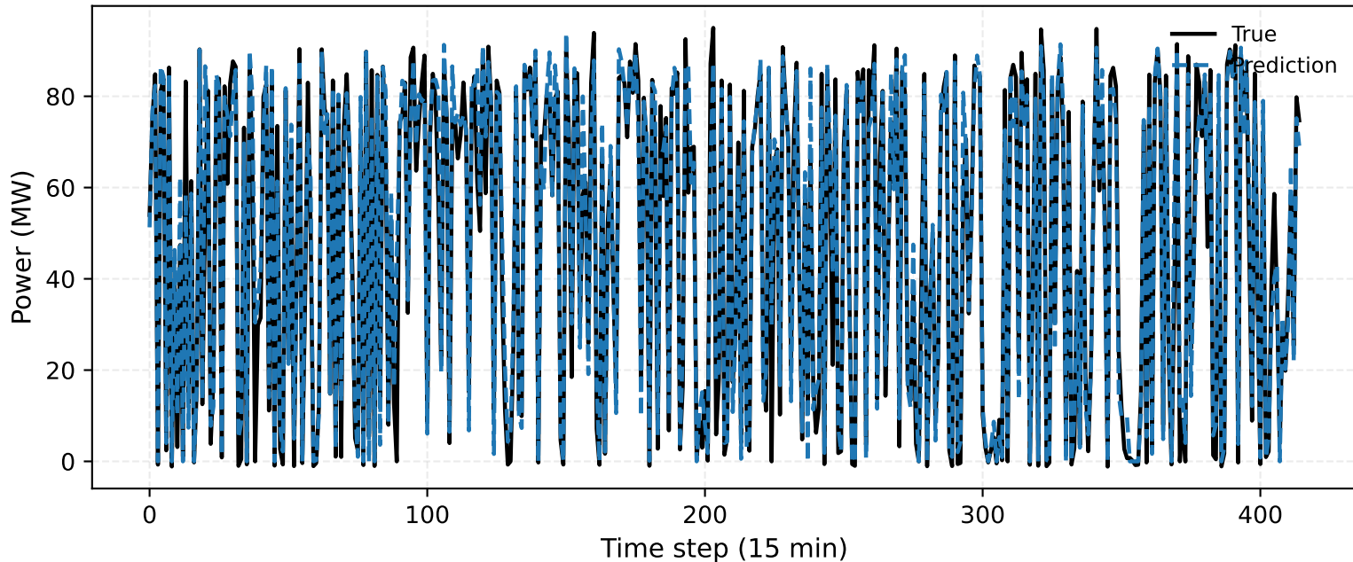
Standard-SVR vs True (Wind farm site 6 (Nominal capacity-96MW)) | Local segment [0, 415)
