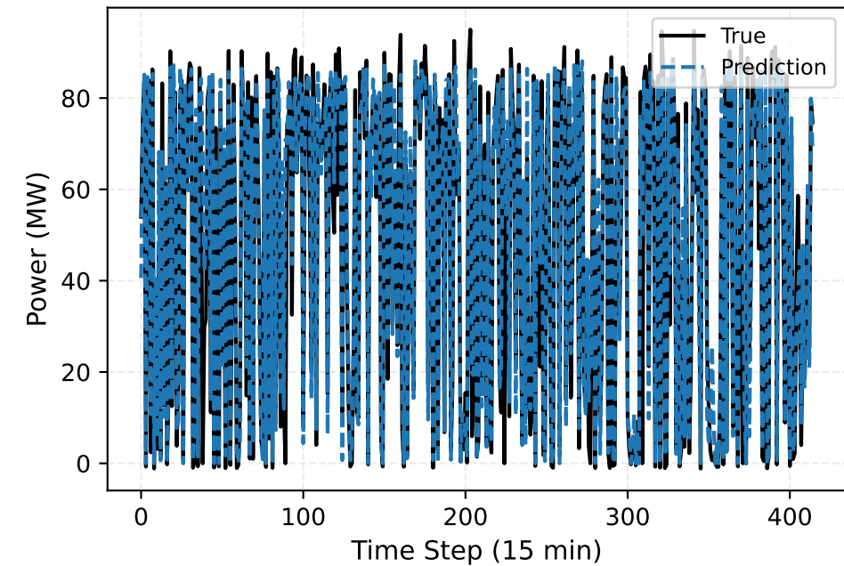
Standard-LDMR vs True (Wind farm site 6 (Nominal capacity-96MW)) Segment [0, 415)
