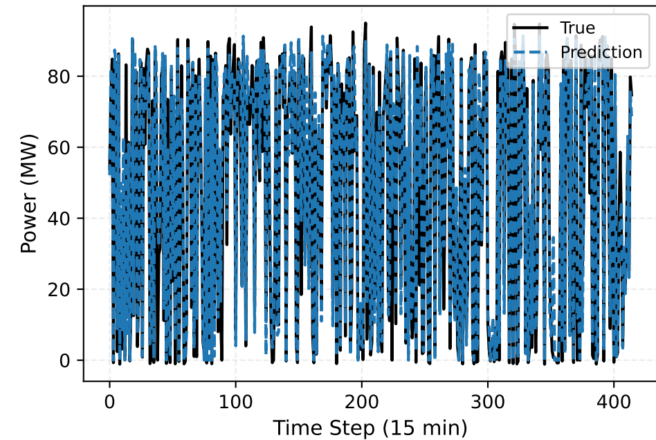
Standard-SVR vs True (Wind farm site 6 (Nominal capacity-96MW)) Segment [0, 415)
